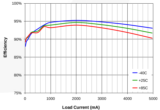
Figure 9. Efficiency vs. I_{LOAD} , 3.3\text{ V}_{OUT}
