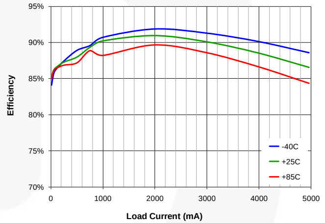
Figure 7. Efficiency vs. I_{LOAD} , 1.8\text{ V}_{OUT}
