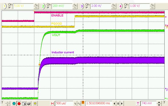
Figure 25. Startup / Shutdown, 240 mΩ Load, C_{OUT}=2\times 22\text{ }\mu\text{F}
