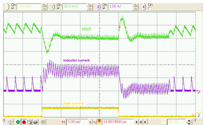
Figure 22. Load Transient, 0.1-1.5 A Load, t_R=t_F=100\text{ ns}
