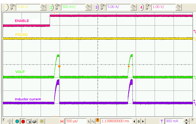
Figure 27. Startup into Overload
