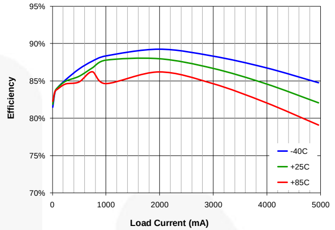
Figure 5. Efficiency vs. I_{LOAD} , 1.2\text{ V}_{OUT}
