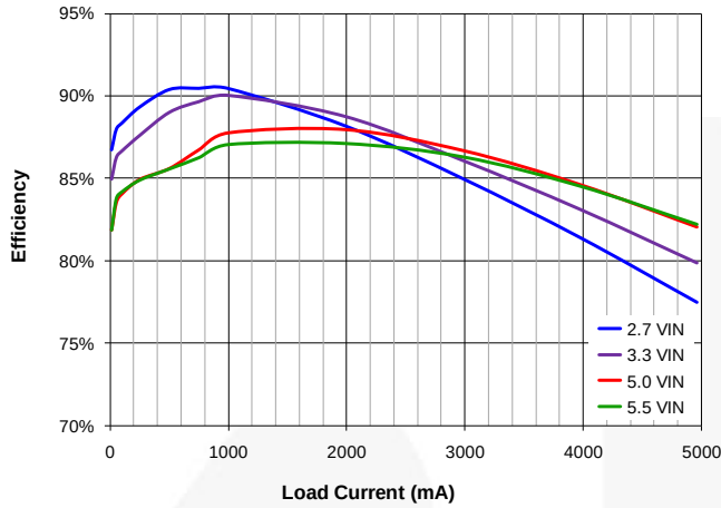
Figure 4. Efficiency vs. I_{LOAD} , 1.2\text{ V}_{OUT}
