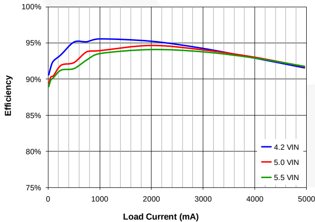
Figure 8. Efficiency vs. I_{LOAD} , 3.3\text{ V}_{OUT}
