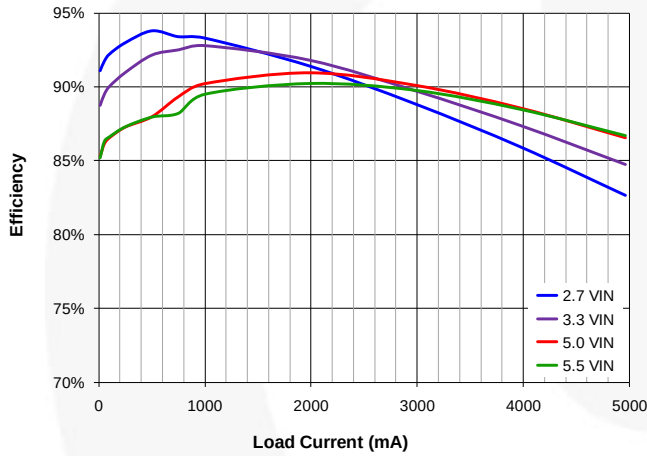
Figure 6. Efficiency vs. I_{LOAD} , 1.8\text{ V}_{OUT}
