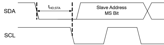
Figure 15. START Bit
