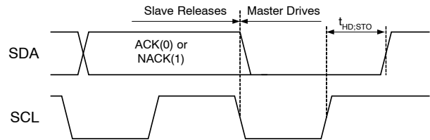
Figure 16. STOP Bit
