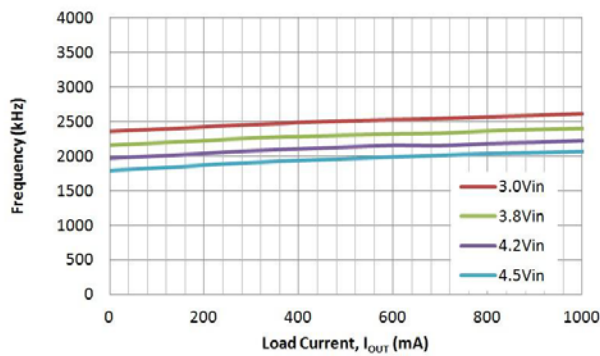
Figure 8. Switching Frequency vs. Load Current and Input Voltage
