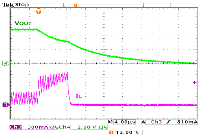
Figure 33. Overload Protection
