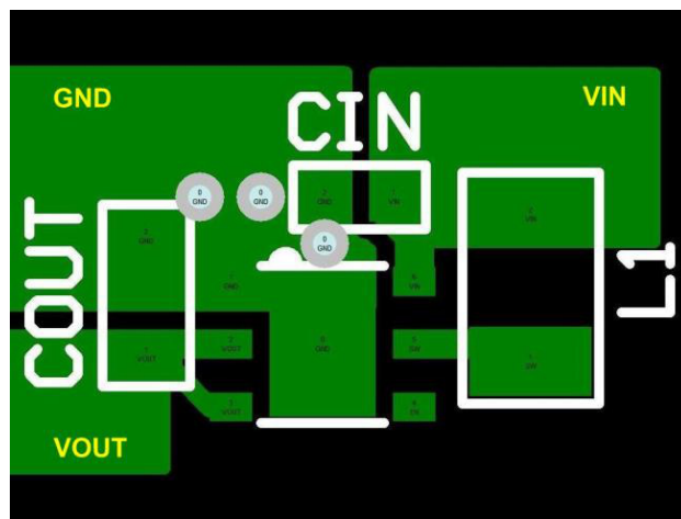
Figure 52. UMLP Suggested Layout (Top View)
