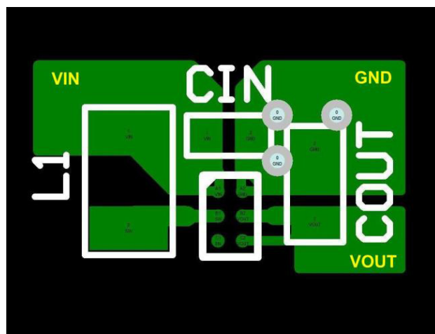
Figure 51. WLCSP Suggested Layout (Top View)
