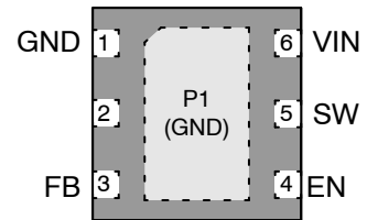
Figure 4. 2x2 mm UMLP (Top View)
