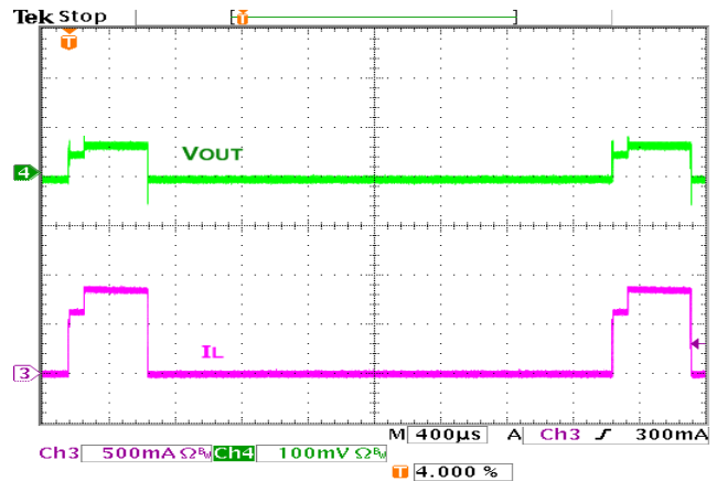
Figure 34. Short-Circuit Response
