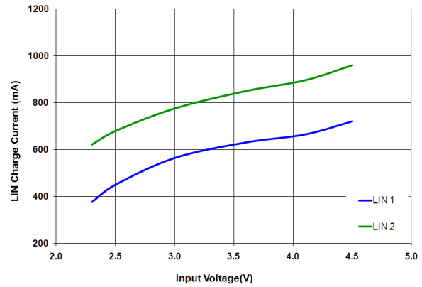
Figure 48. LIN Mode Current vs. V_{IN}
