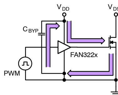
Figure 48. Current Path for MOSFET Turn-On
