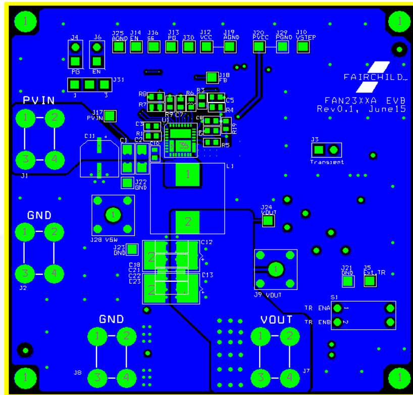
Figure 26. Evaluation Board Top Layer Copper
