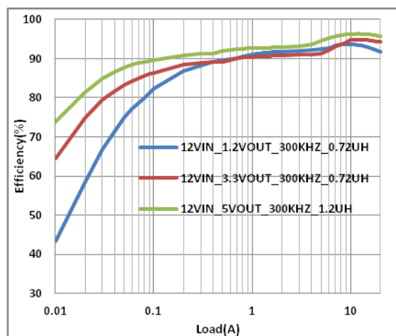
Figure 7. Efficiency vs. Load Current with V_{IN}=12 V and f_{SW}=300 kHz
