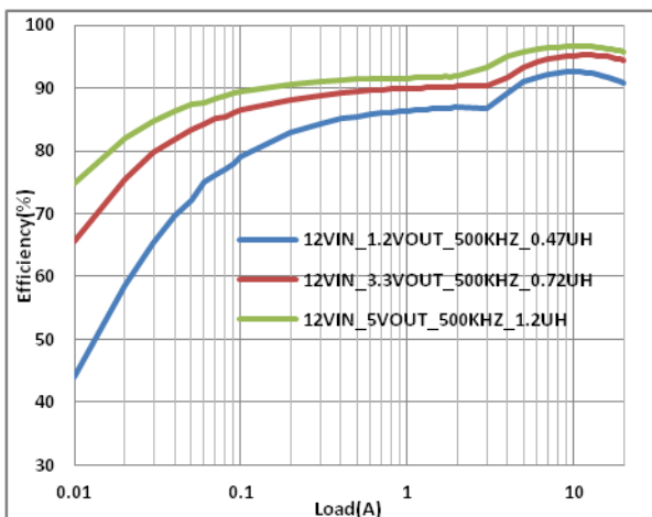
Figure 6. Efficiency vs. Load Current with V_{IN}=12 V and f_{SW}=500 kHz
