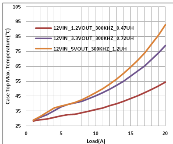
Figure 9. Case Top Temperature vs. Load Current with V_{IN}=12 V and f_{SW}=300 kHz
