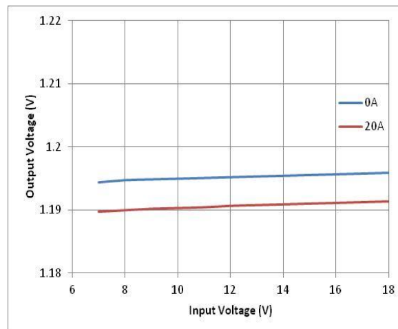
Figure 11. Line Regulation with V_{IN}=12 V, V_{OUT}=1.2 V and f_{SW}=500 kHz
