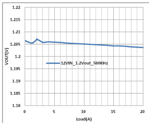
Figure 10. Load Regulation with V_{IN}=12 V, V_{OUT}=1.2 V and f_{SW}=500 kHz
