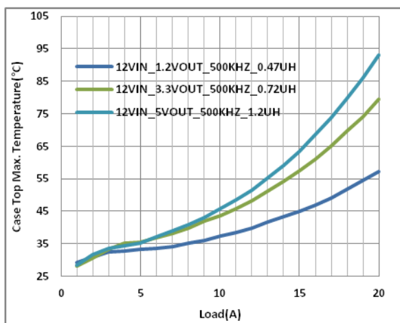
Figure 8. Case Top Temperature vs. Load Current with V_{IN}=12 V and f_{SW}=500 kHz
