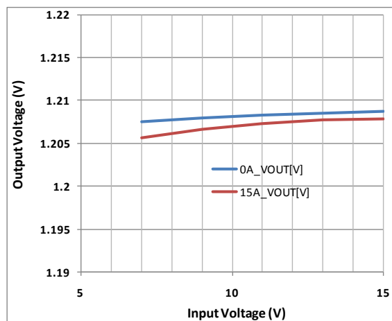
Figure 11. Line Regulation
