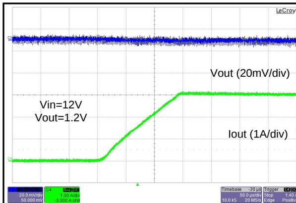
Figure 23. FAN23SV06PA Operation as Load Changes from 0 A to 3 A
