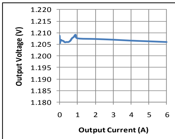
Figure 12. Load Regulation
