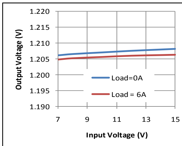
Figure 13. Line Regulation
