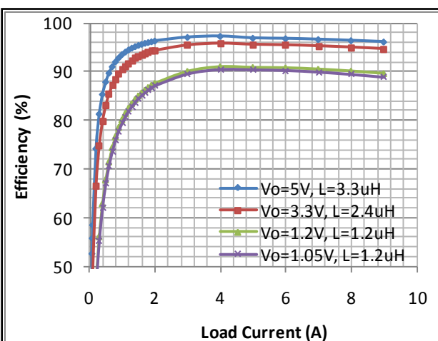
Figure 9. FAN23SV06PA Efficiency vs. Load Current V_{IN}=12\text{ V} and f_{SW}=500\text{ kHz}
