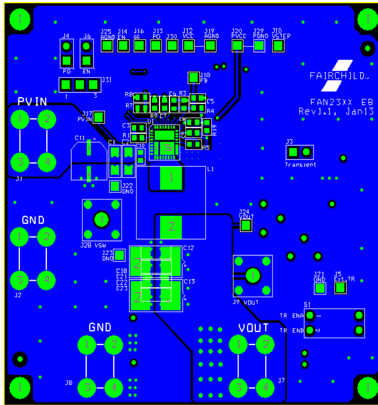
Figure 30. Evaluation Board Top Layer Copper
