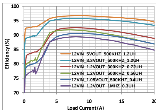
Figure 10. Efficiency vs. Load Current with V_{IN}=12\text{ V}
