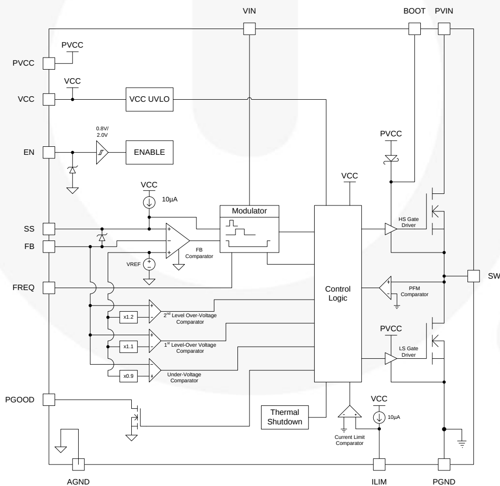
Figure 2. Block Diagram
