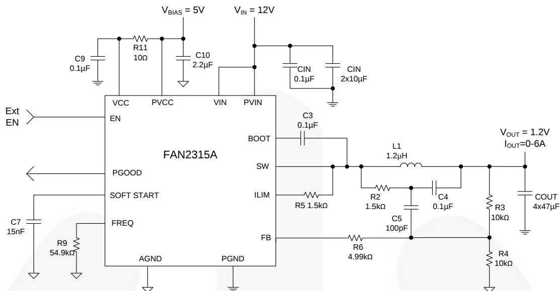
Figure 1. Typical Application
