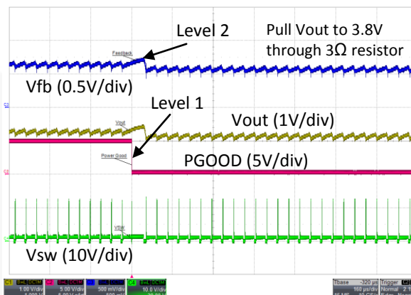
Figure 23. Over-Voltage Protection Level 1 and Level 2
