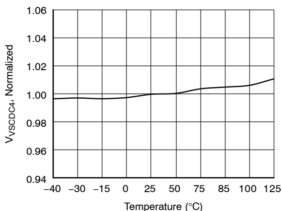
Figure 17. Cable Compensation Level 4 Reference Voltage ( V_{VS-CD4} ) vs. Temperature
