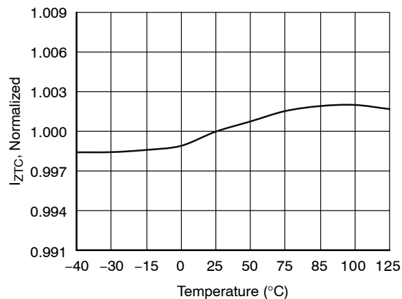
Figure 16. Dynamic Trigger Current Threshold ( I_{ZTC} ) vs. Temperature
