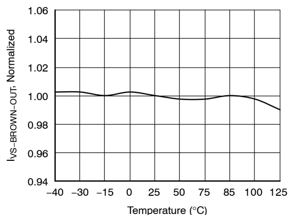
Figure 20. Brown Out Threshold Current ( I_{VS-BROWN-OUT} ) vs. Temperature
