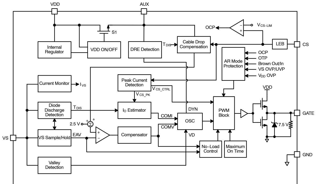
Figure 2. FAN105A Function Block Diagram
