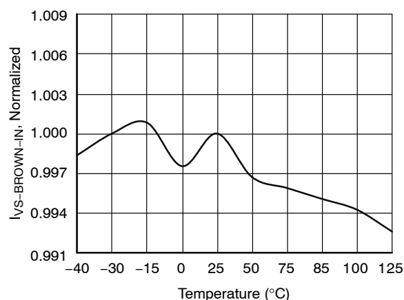
Figure 18. Brown In Threshold Current ( I_{VS-BROWN-IN} ) vs. Temperature
