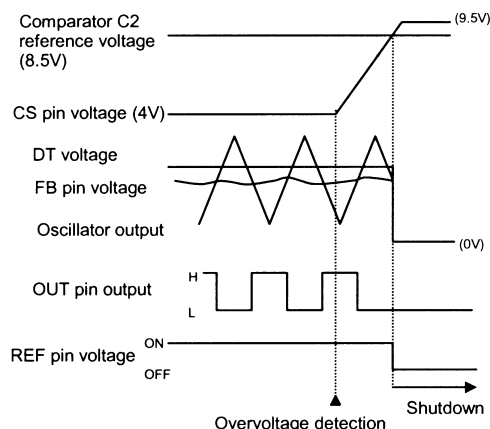
Fig. 17 Overvoltage shutdown timing chart
