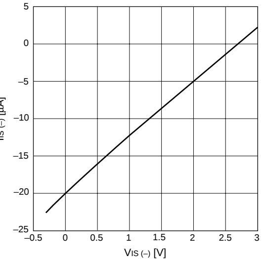
IS (-) terminal current (Iis (-)) vs. IS (-) terminal voltage (Vis (-)) FA3647
