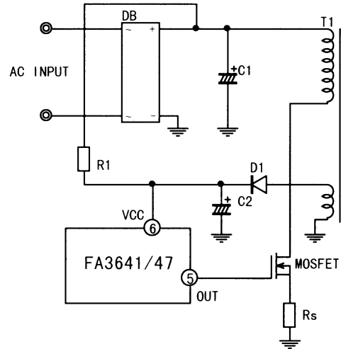
Fig. 20 Startup circuit (2)
