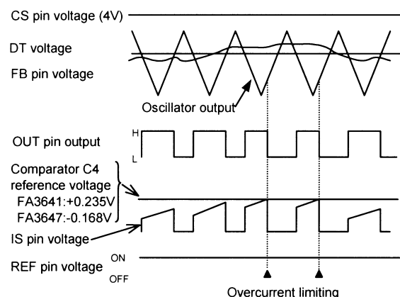
Fig. 15 Overcurrent timing chart
