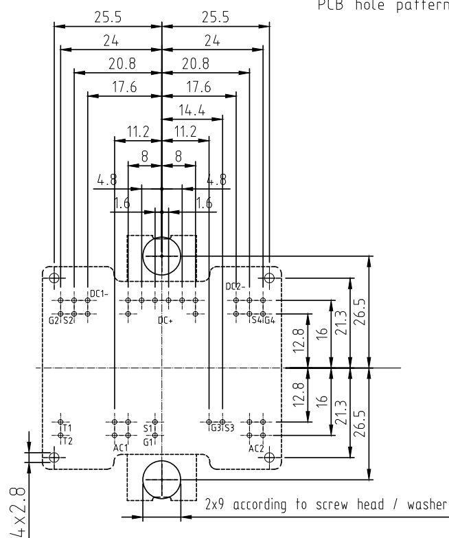
PCB hole pattern
