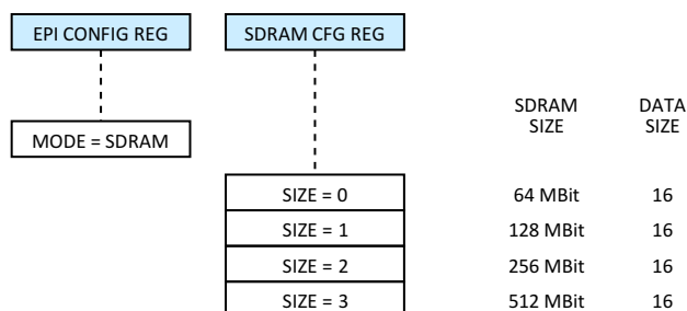
Figure 7-9. EPI SDRAM Mode
