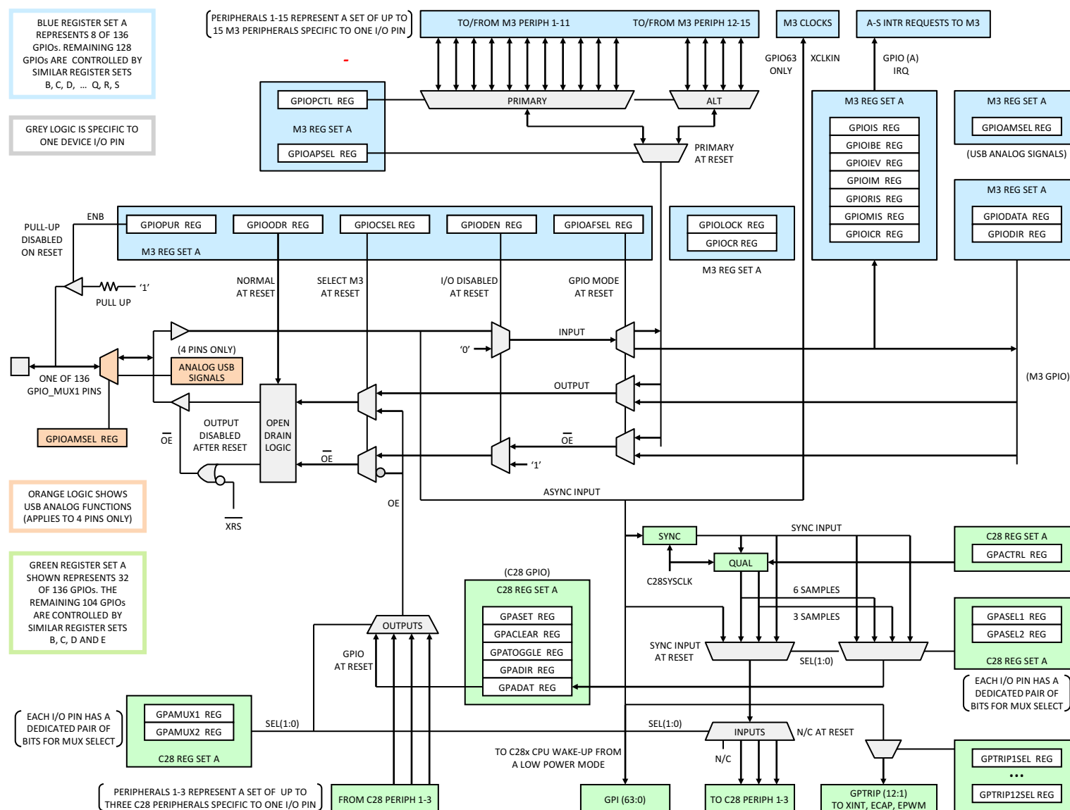
Figure 3-16. GPIO MUX1 Pin Mapping Through Register Set A
