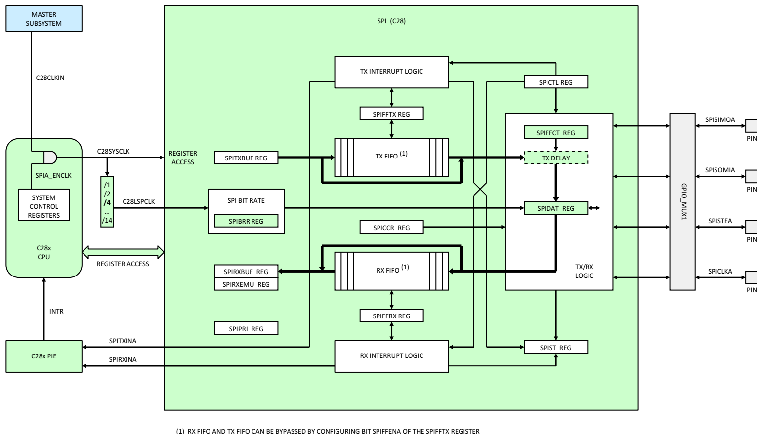
Figure 7-41. SPI (C28x)
