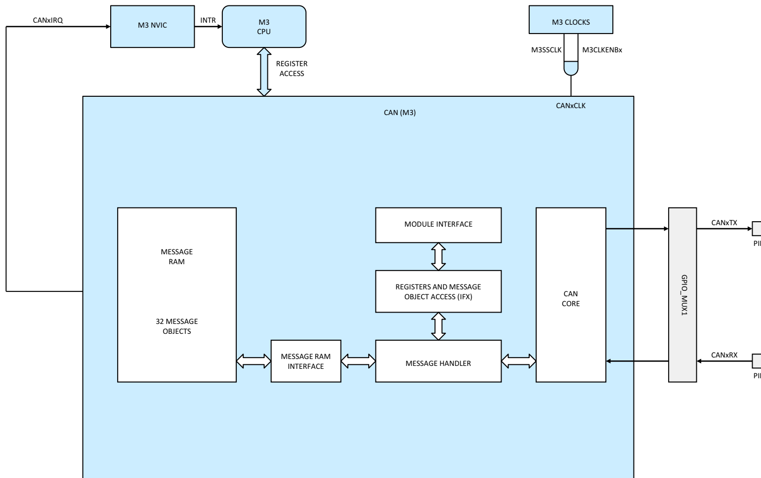
Figure 7-24. CAN (Cortex-M3)
