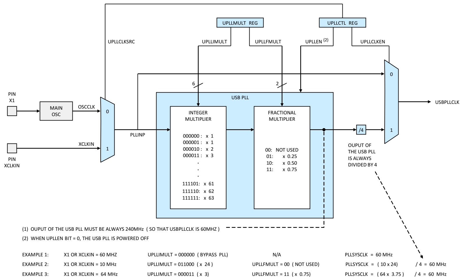
Figure 3-9. USB PLL
