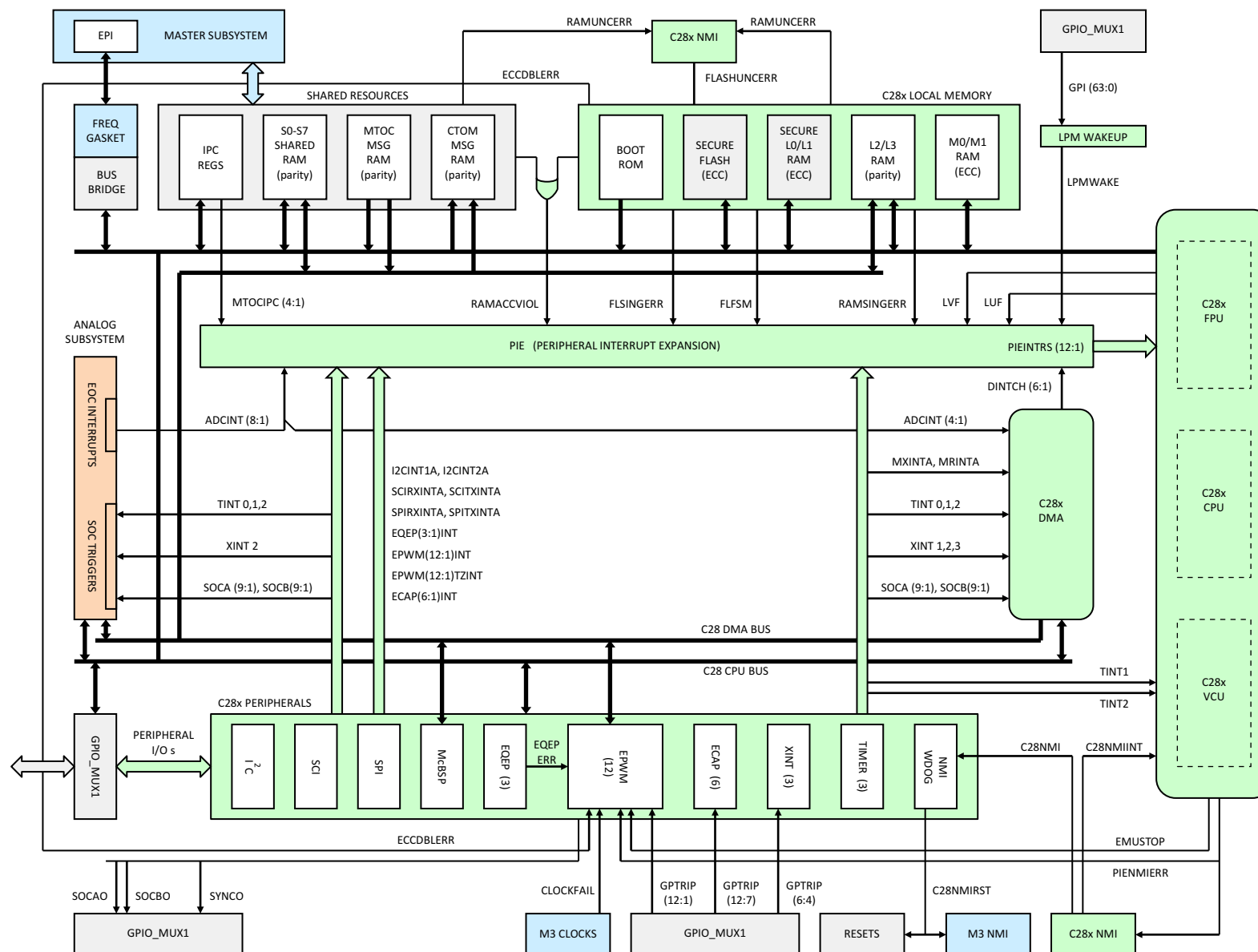
Figure 3-2. Control Subsystem
