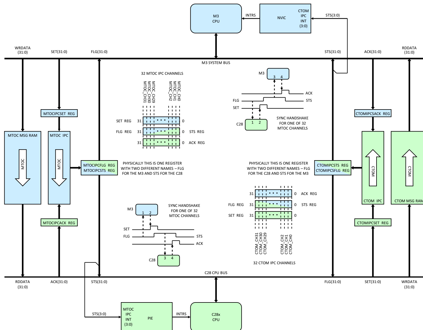
Figure 7-6. IPC
