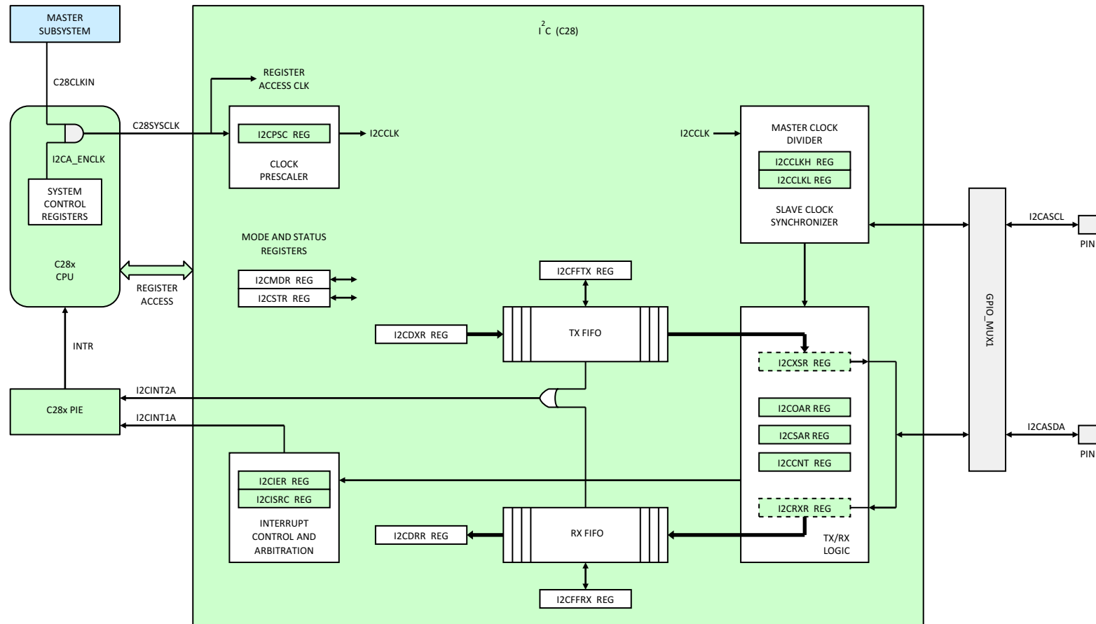
Figure 7-39. I²C (C28x)
