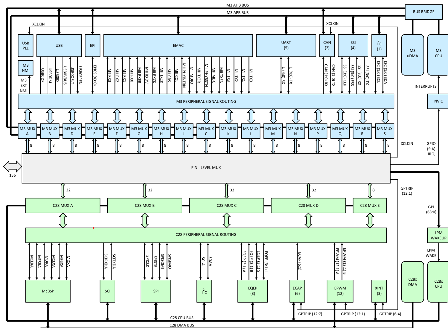
Figure 3-15. GPIO_MUX1 Block
