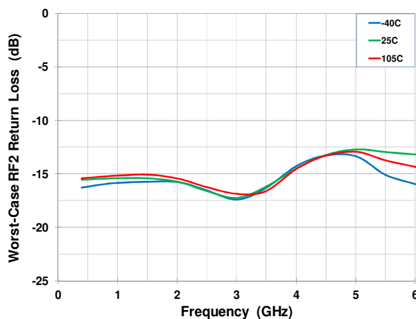
Figure 29. Worst-Case Return Loss (ATTEN_RF2 port) vs. Frequency over Temp
