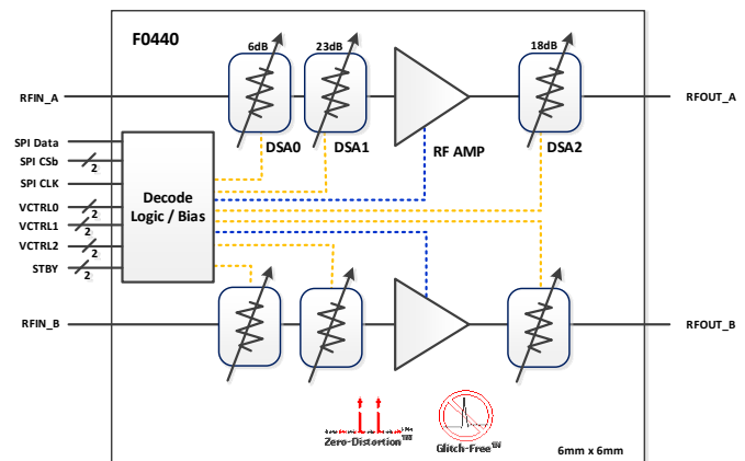
Figure 1. Block Diagram
