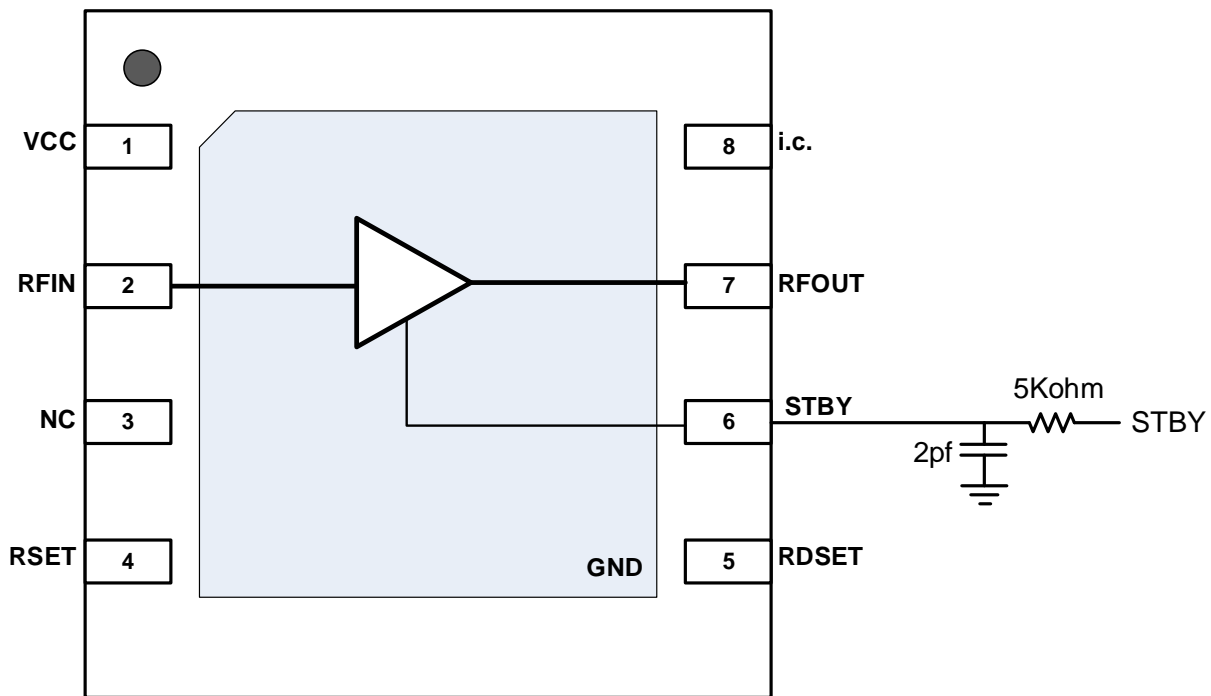
Figure 42. Control Pin Interface for Signal Integrity
