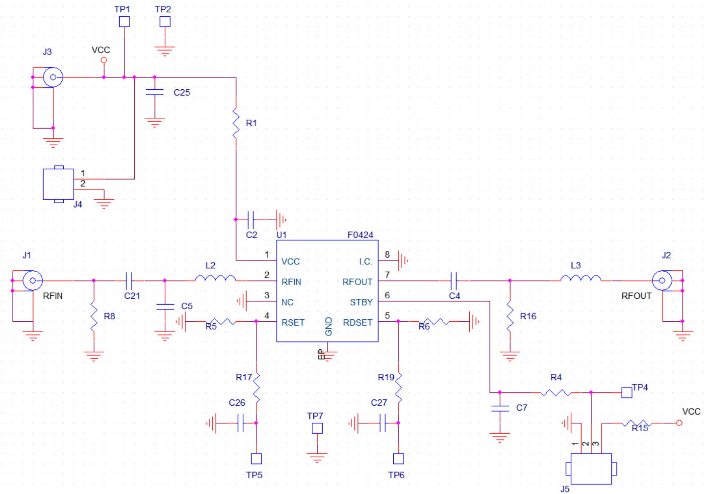
Figure 41. Electrical Schematic
