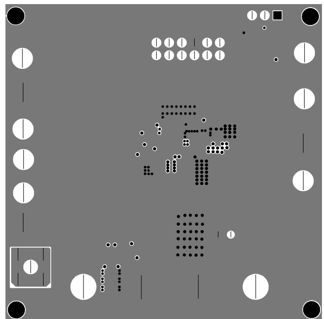
Figure 4-Inner1 Layer
