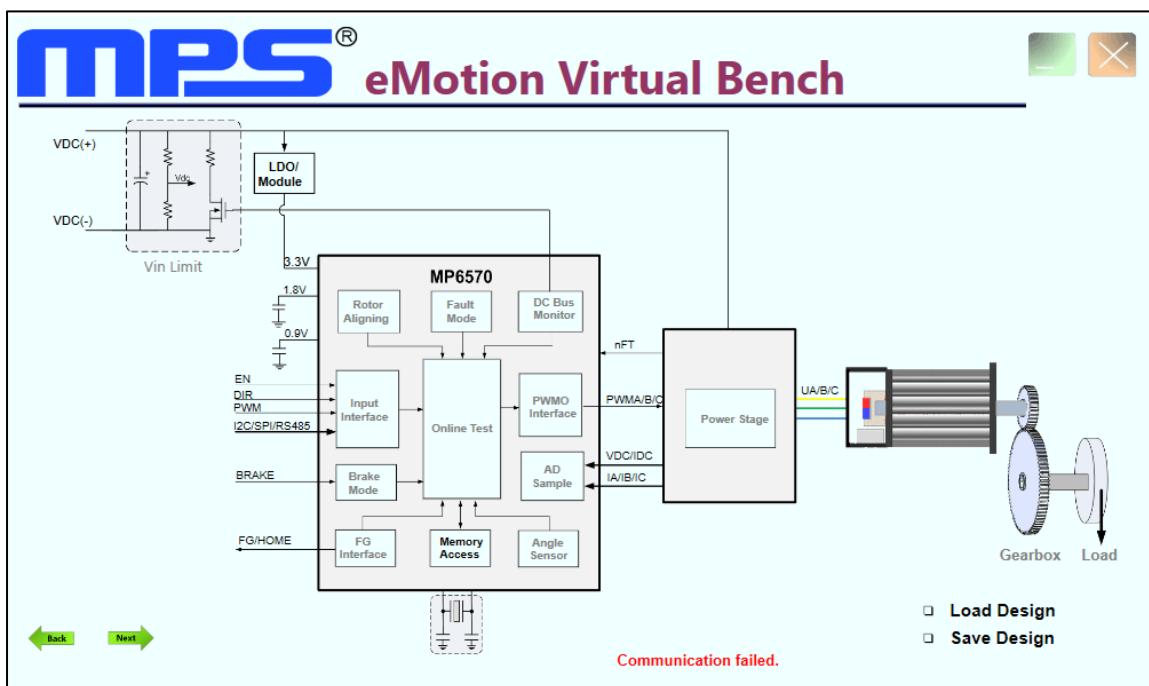
Figure 7: Connection Status
