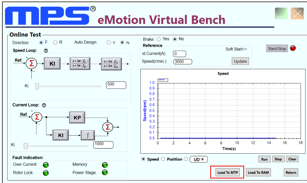
Figure 12: Write MTP
