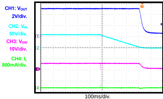
Power Off I_{OUT}=0A
