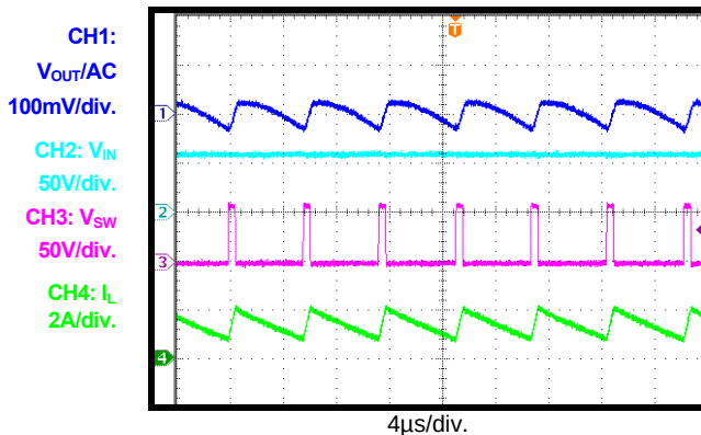
Steady State I_{OUT}=1A
