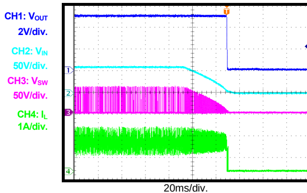
Power Off I_{OUT}=1A
