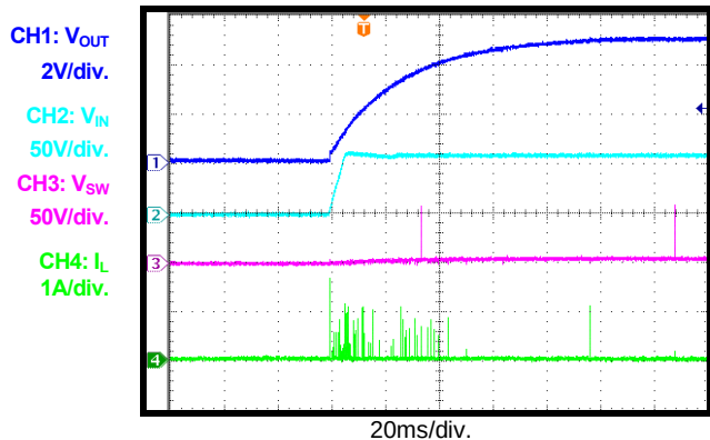
Power On I_{OUT}=0A
