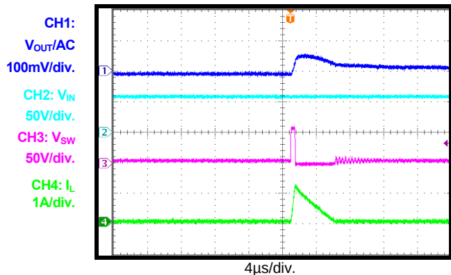
Steady State I_{OUT}=0A
