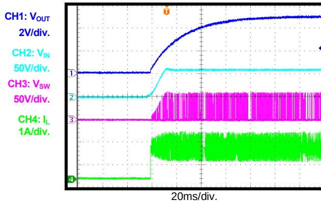
Power On I_{OUT}=1A
