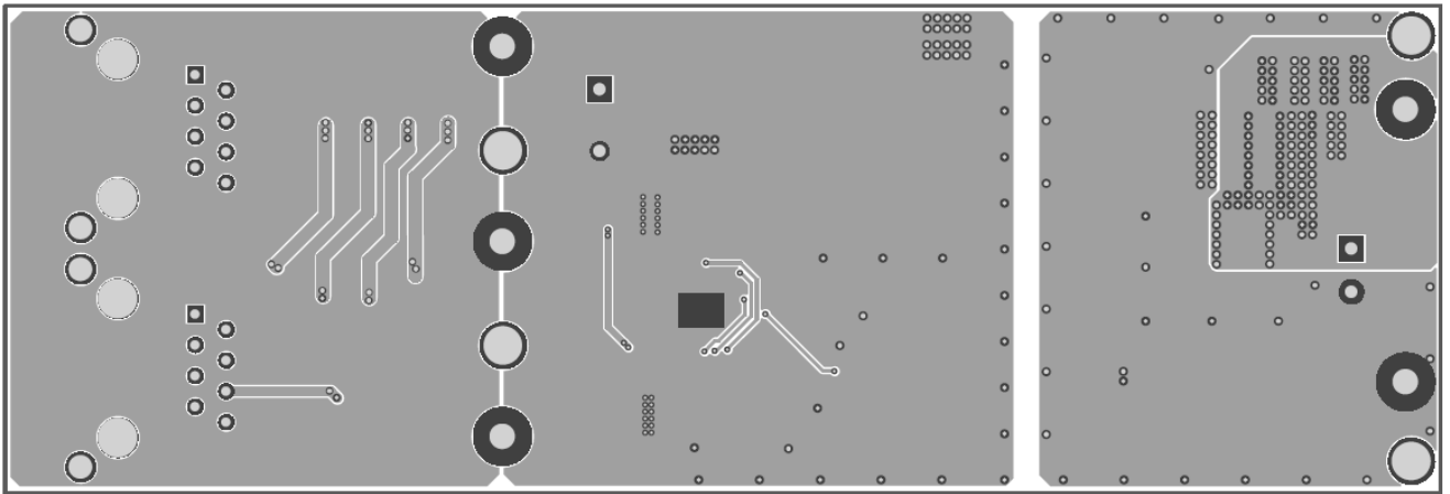
Figure 3: Bottom Layer
