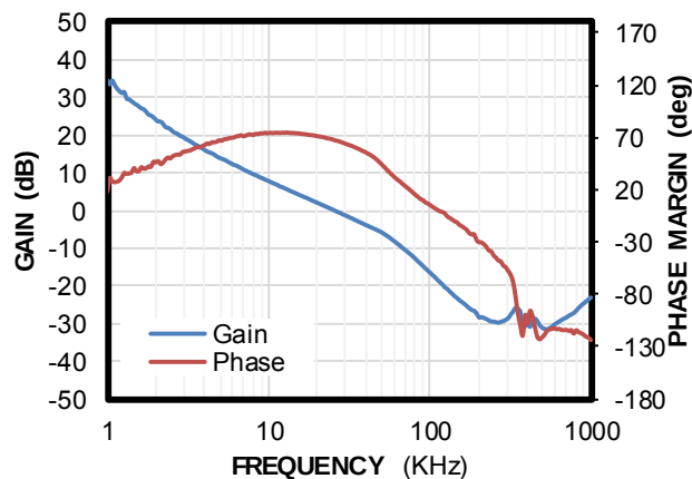
Bode Plot
