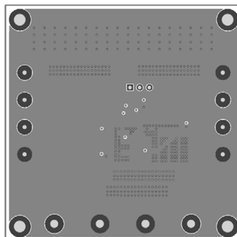
Figure 4—Inner Layer 2
