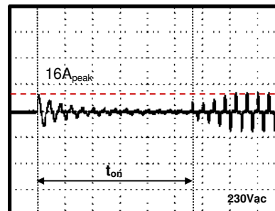
(Fig.8 inrush with an ESB)
