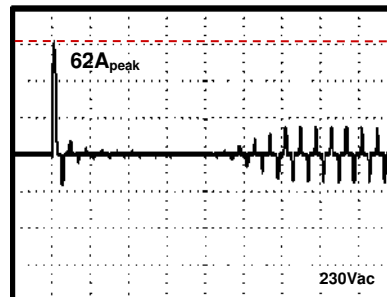
(Fig.7 inrush without an ESB)
