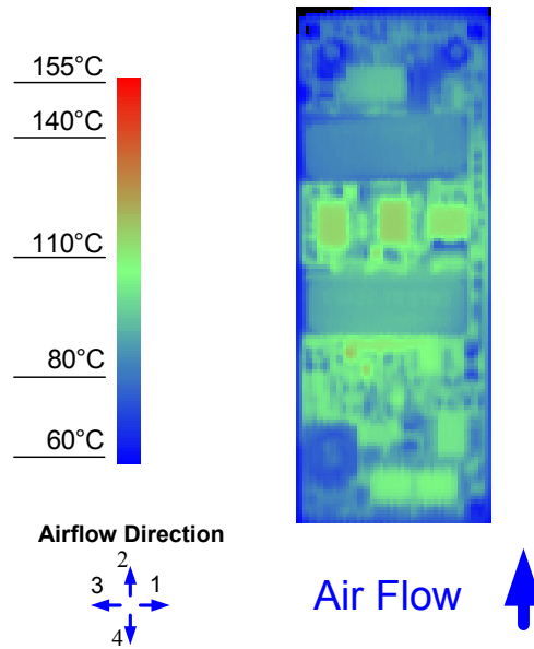
Figure 14. Thermal Image for Airflow Direction 2 (18.7A output, 55°C ambient, 200 LFM, V_{in} = 48V open frame unit soldered into fixture board)
