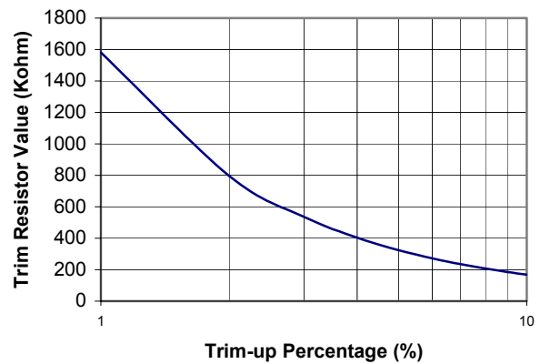
Fig. 19 Trim-Up Resistor Selection
