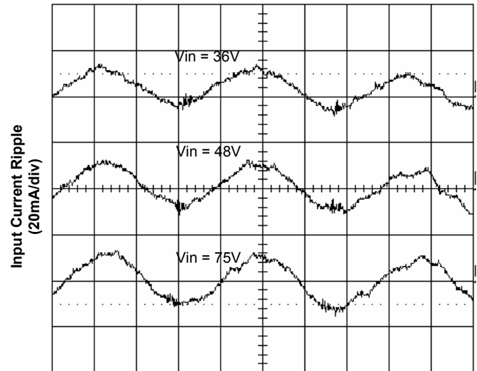
Time - t (1µs/div) Figure 6. Input Reflected Ripple Current at 20A Load
