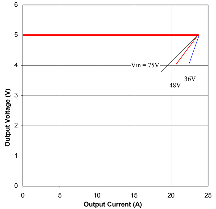
Figure 10. Output Characteristics
