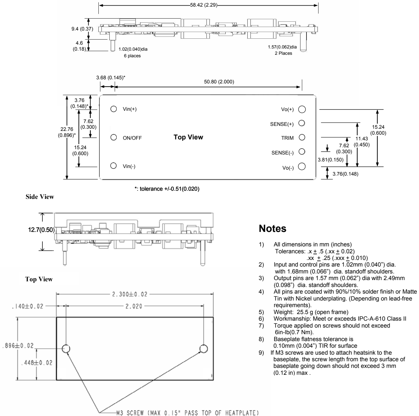
Figure 20. Converter with optional baseplate
