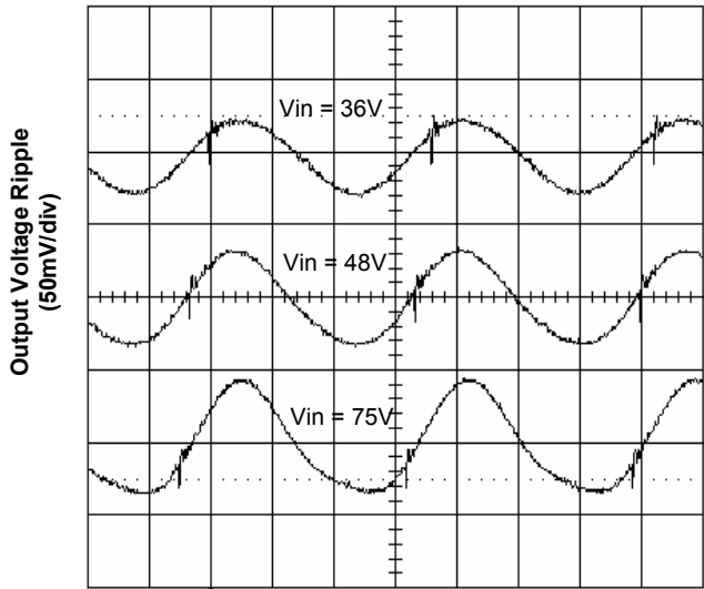
Time - t (1µs/div) Figure 5. Output Ripple Voltage at 20A Load
