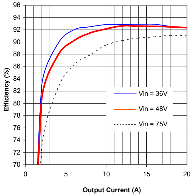
Figure 1. Efficiency vs. Load Current (25°C)
