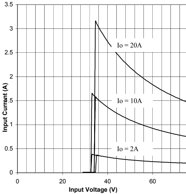
Figure 9. Input Characteristics
