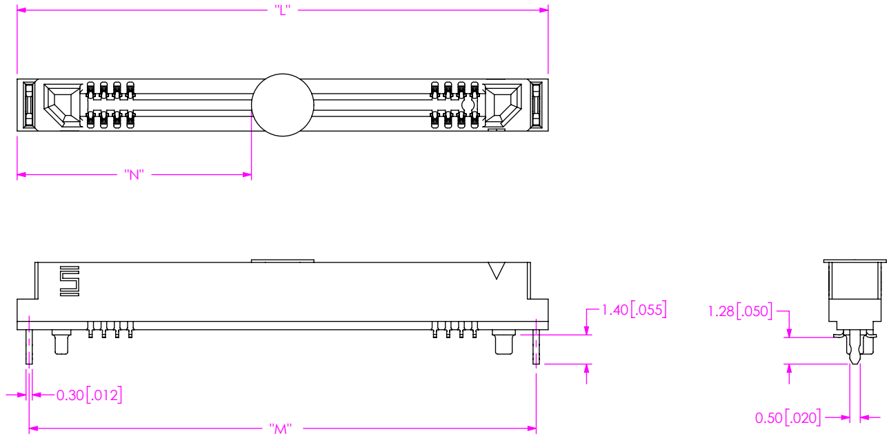
FIG 2 ERF6-30-03.5-X-DV-A-WT-K-XR SHOWN (DIFFERENT AS SHOWN, OTHERWISE SAME AS FIG 1) (SOME CENTER FEATURES REMOVED FOR CLARITY)
