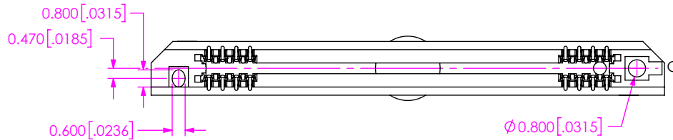
FIG 1 ERF6-30-03.5-X-DV-A-K-XR SHOWN (SOME CENTER FEATURES REMOVED FOR CLARITY)
