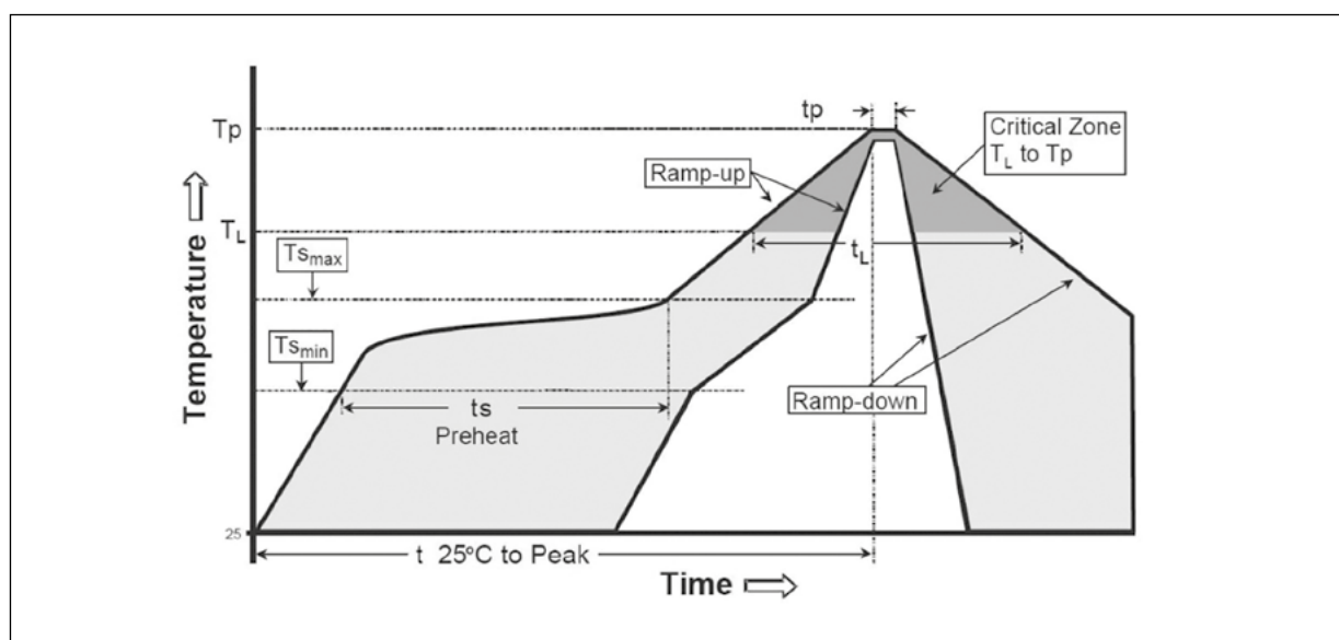
Figure 36: Soldering Recommendations
