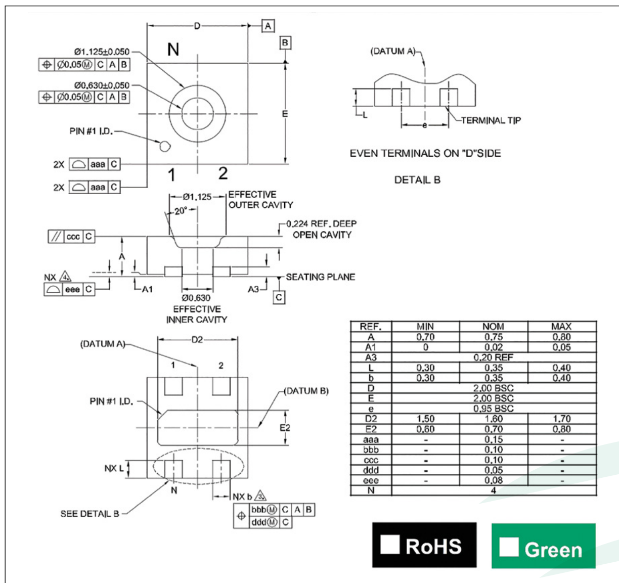
Figure 39: Package Outline
