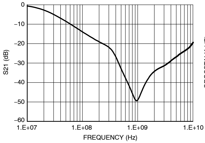
Figure 1. Typical Insertion Loss
