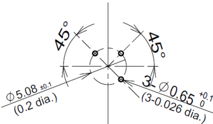
Recommended PCB Pattern Diagram
