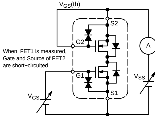
Figure 13. Test Circuit 3
