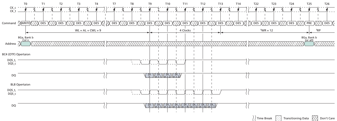
Figure 179: WRITE (BL8/BC4-OTF) to PRECHARGE with 1t_{CK} Preamble
