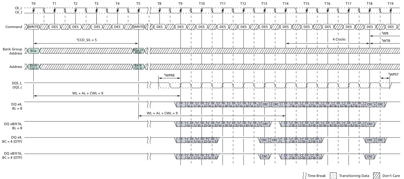
Figure 186: Consecutive WRITE (BL8/BC4-OTF) with 1 st CK Preamble and Write CRC in Same or Different Bank Group
