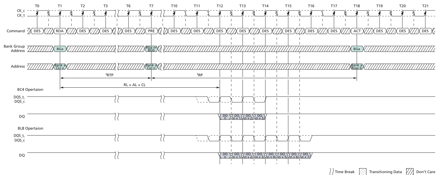
Figure 145: READ with Auto Precharge and 1^{tCK} Preamble
