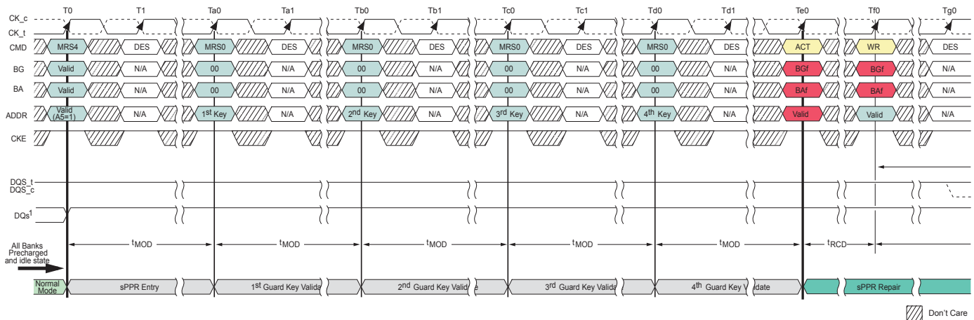
Figure 69: sPPR – Entry
