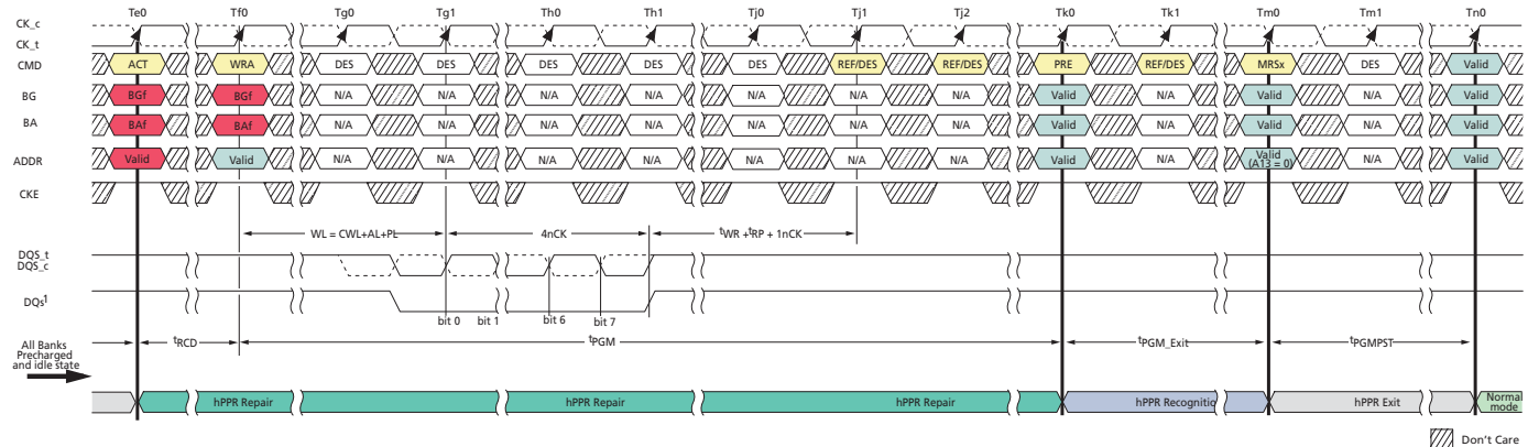
Figure 66: hPPR WRA – Repair and Exit
