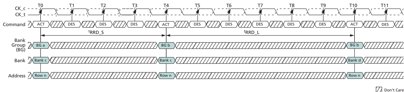
Figure 71: t_{RRD} Timing
