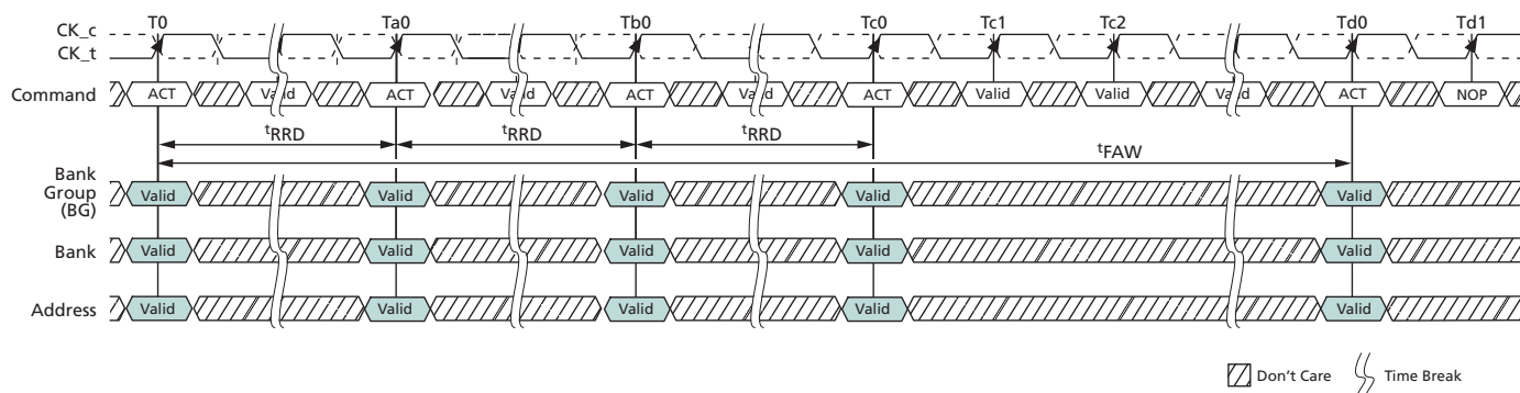
Figure 72: t_{FAW} Timing
