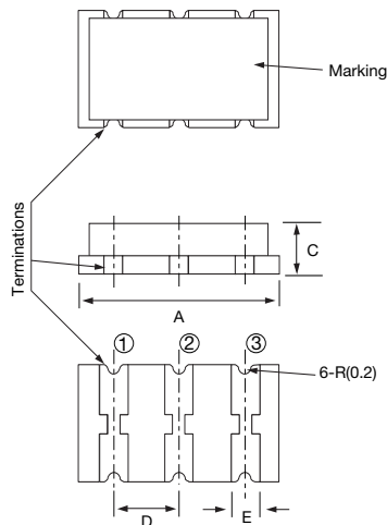
Figure 1) ECS-SR-B Series - Top, Side, Bottom & End views
