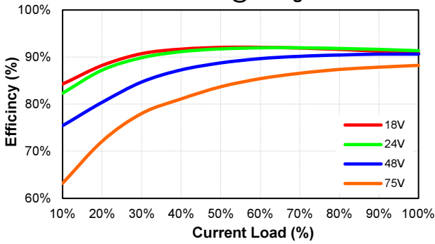
ECLB60W-48S33 Eff Vs Io @25 Deg. C
