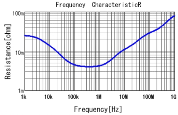
■ ECASD60J157M010K00 R DCOV, 25degC
