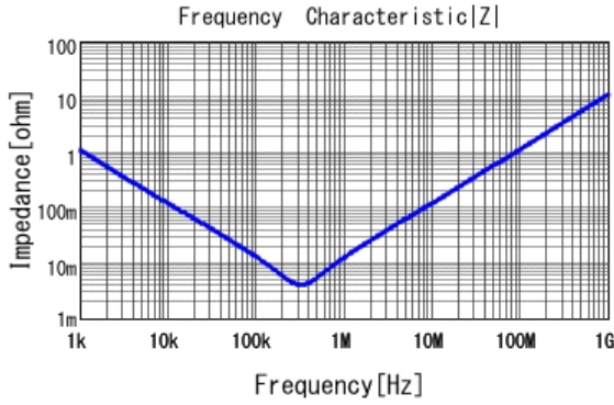
■ ECASD60J157M010K00 |Z| DCOV, 25degC
