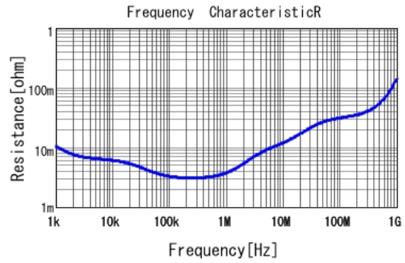
■ ECASD60E477M4R5K00 R DCOV, 25degC
