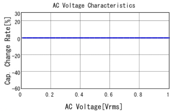
■ ECASD60E477M4R5K00 C-AC Voltage capchange, DCOV, 25.0
