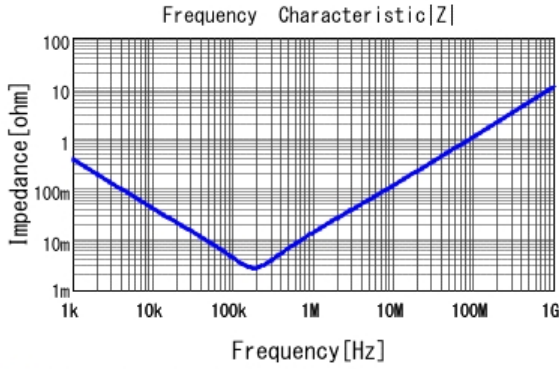
■ ECASD60D477M4R5K00 |Z| DC0V, 25degC
