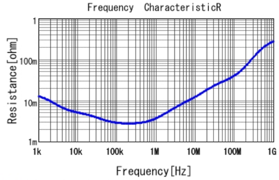
■ ECASD60D477M4R5K00 R DC0V, 25degC
