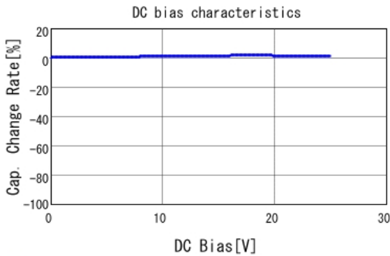
■ ECASD41E226M040KA0 C-DC bias capchange, 25.0degC, AC1
