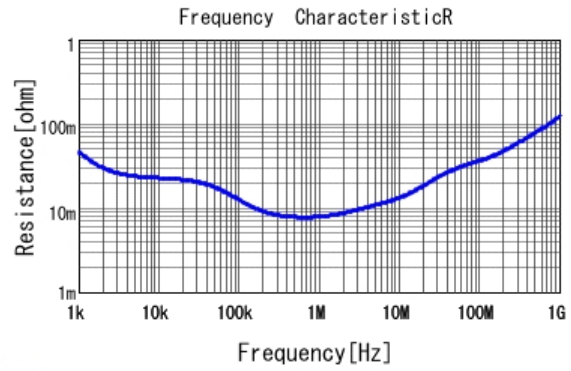
■ ECASD41C476M040KA0 R DCOV, 25degC
