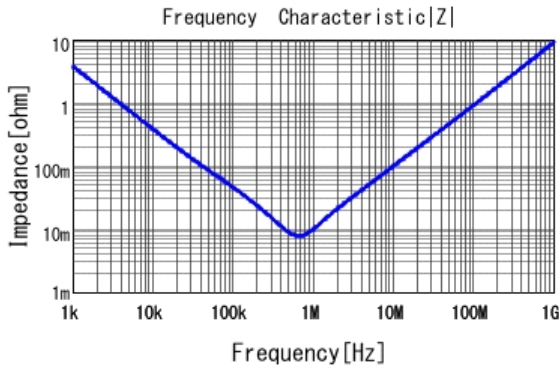
■ ECASD41C476M040KA0 |Z| DCOV, 25degC
