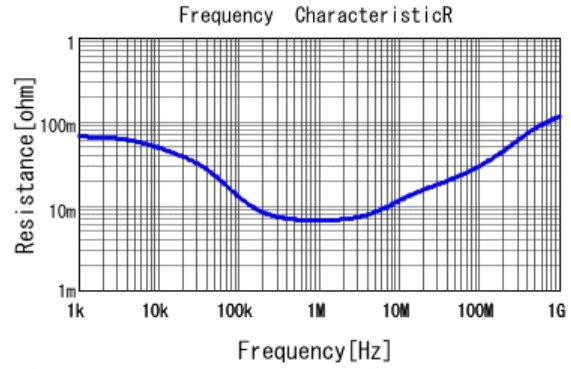
■ ECASD40J336M025K00 R DCOV, 25degC
