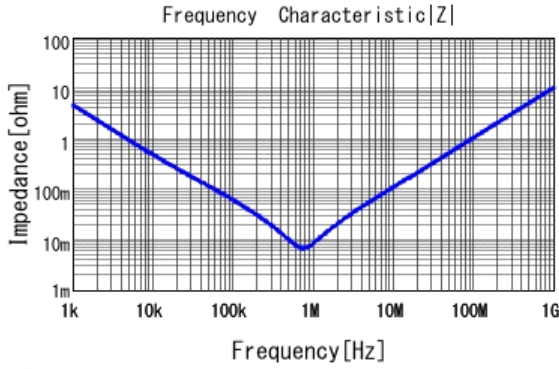
■ ECASD40J336M025K00 |Z| DCOV, 25degC
