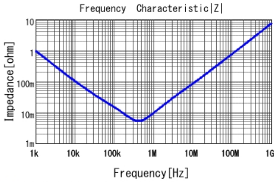
■ ECASD40J157M015K00 |Z| DCOV, 25degC
