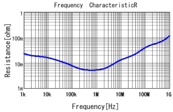
■ ECASD40J157M015K00 R DCOV, 25degC
