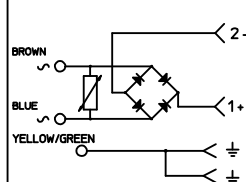
ELECTRICAL DIAGRAM S3
