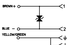
ELECTRICAL DIAGRAM S1
