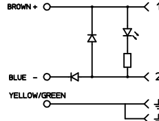
ELECTRICAL DIAGRAM 00
