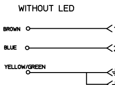
ELECTRICAL DIAGRAM 00
