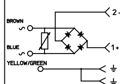
ELECTRICAL DIAGRAM S3
