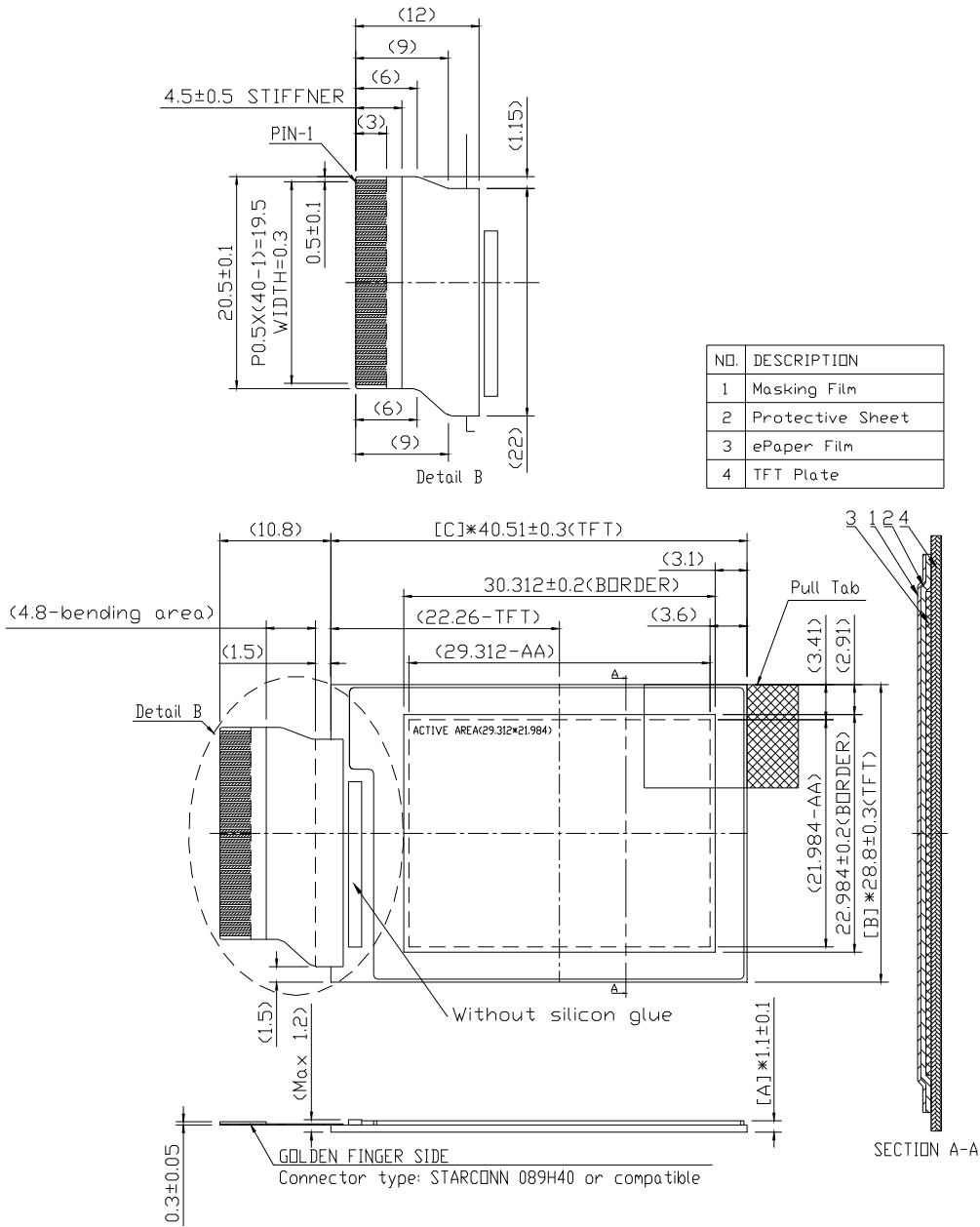
Figure 1-1 EPD Drawing
