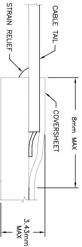
SECTION B-B NTS
