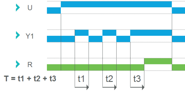
Function Tt - Delayed Latching (Alternating) – Leading Edge
