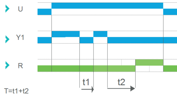
Function Bw - Pulse output
