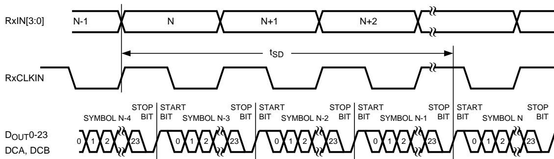
Figure 9. Latency Delay
