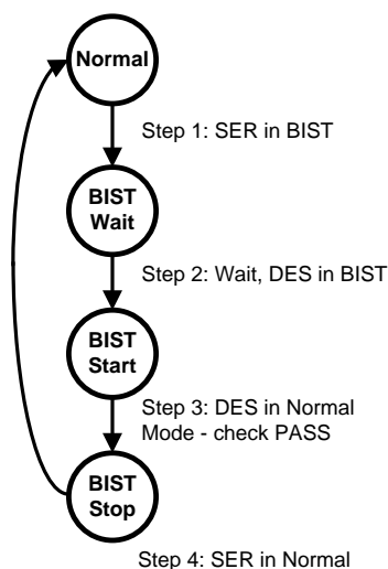
Figure 20. BIST Mode Flow Diagram
