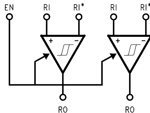
Figure 2. Function Diagram
