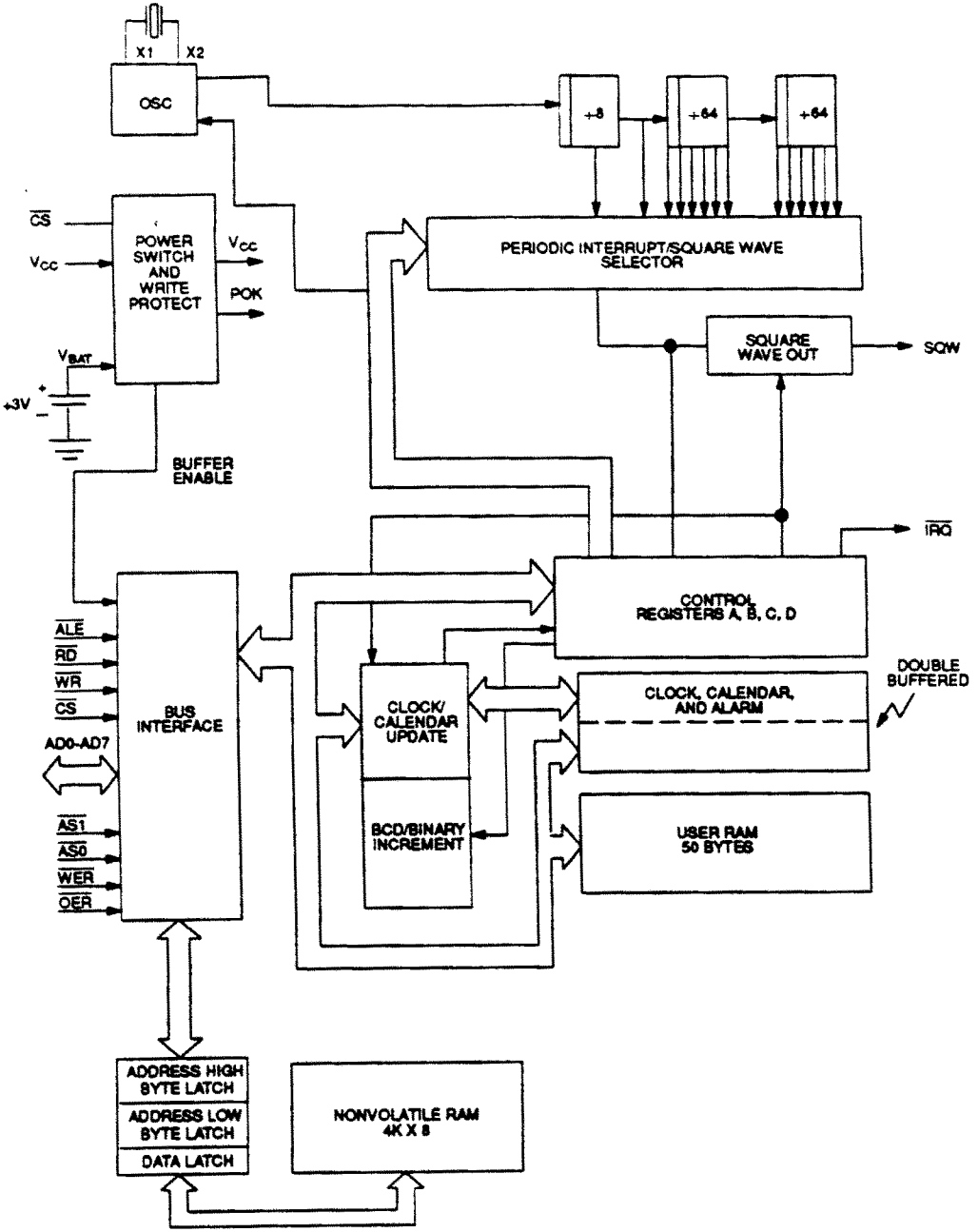
DS1385/DS1387 BLOCK DIAGRAM Figure 1
